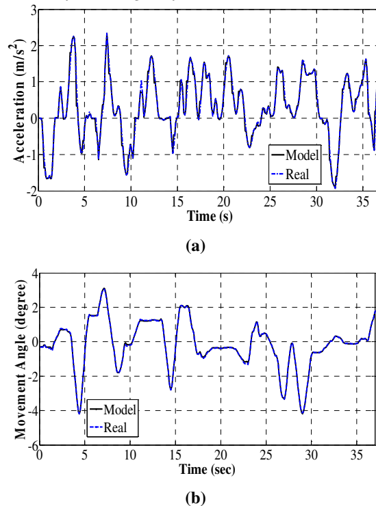
Fig8. Comparison of the MANFIS model and real data: (a) longitudinal acceleration, (b) Movement Angle.
