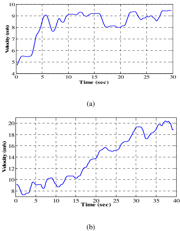
Fig13. Comparison of the range of velocities, (a) test vehicle of Fig. 7, (b) test vehicle of Fig. 9.
