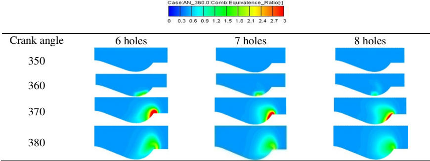
Fig12. 2D contour of equivalence ratio in different crank angle for injectors
