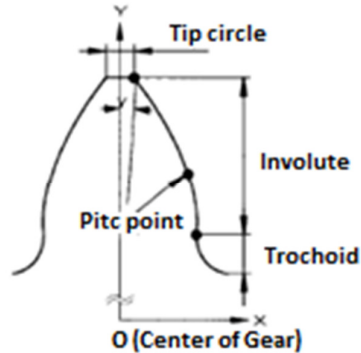
Fig5. Coordinate system of an involute tooth profile
