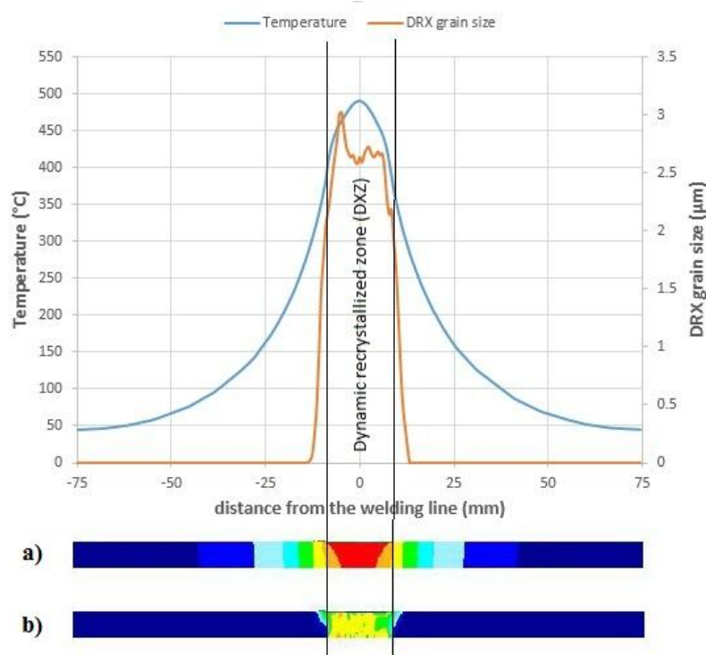
Fig2. temperature (a) and dynamically recrystallized grain size (b) profile and distribution in a transverse section of welded plates
