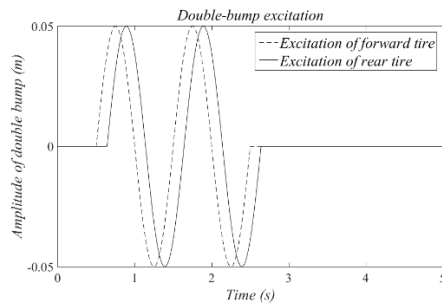
Figure 12. Double-bump excitation [10, 12].
