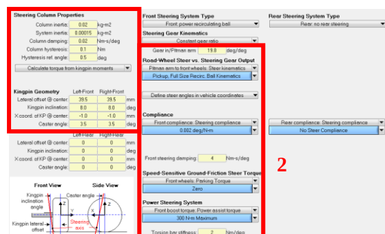
Figure30: CarSim Steering System Section
