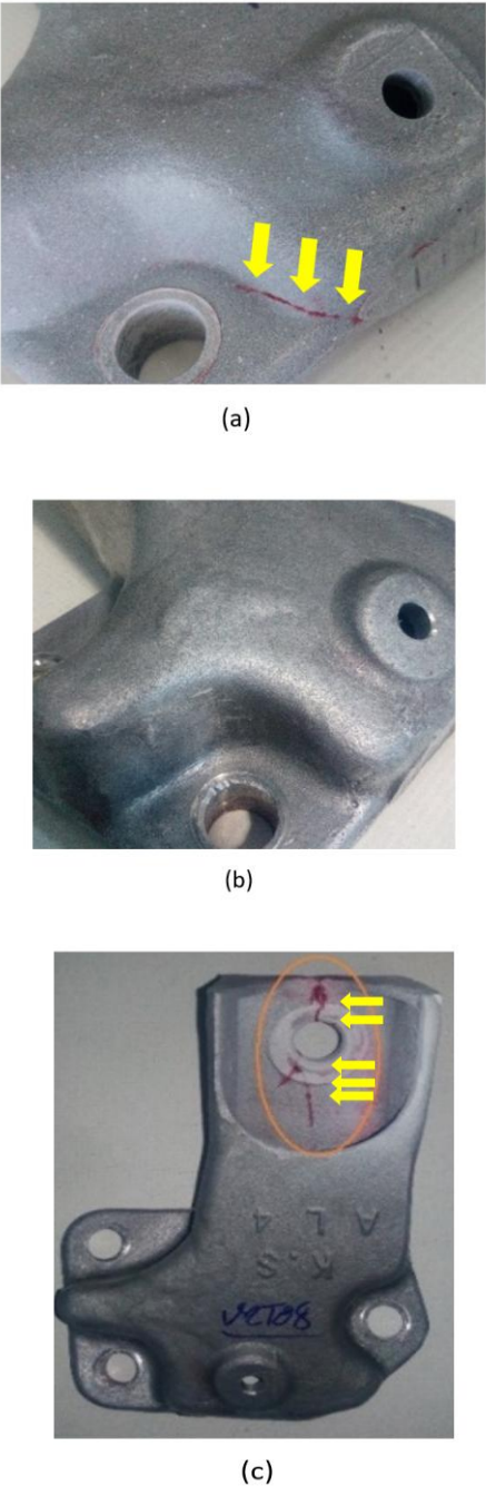
Figure 11. a) Identification of the crack in the front area of the primary sample. b) Removal of the crack in the front area of the modified sample. c) Appearance of a crack in the end area of the modified sample.
