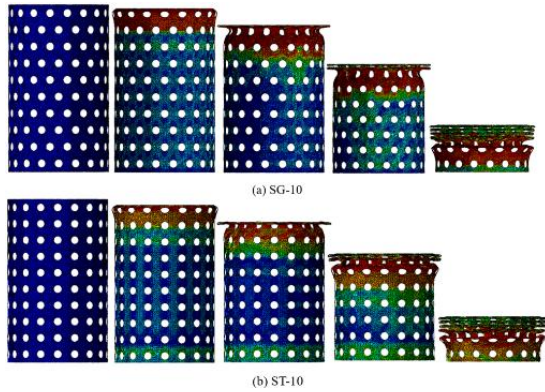
Figure 22: Deformation patterns of (a) SG-10 and (b) ST-10
