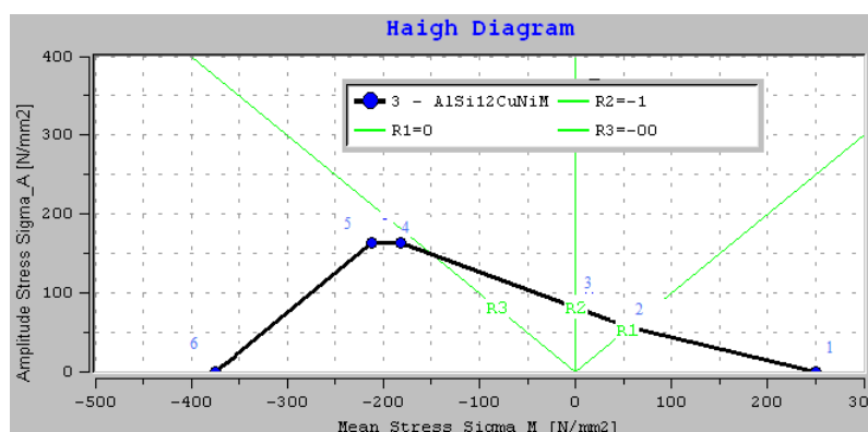
Fig. 9. Haigh diagram of piston material [11].
