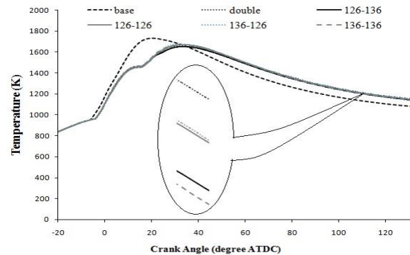
Fig 8. In-cylinder temperature for the cases that below row injected first
