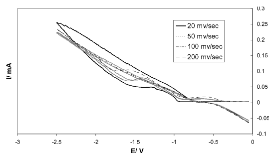
Fig. 2. Cyclic voltammogram for cobalt deposition on the platinum surface from sulfate-borate solution, \Psi=20, 50, 100 and 200 \text{ mVs}^{-1} (ambient temperature).
