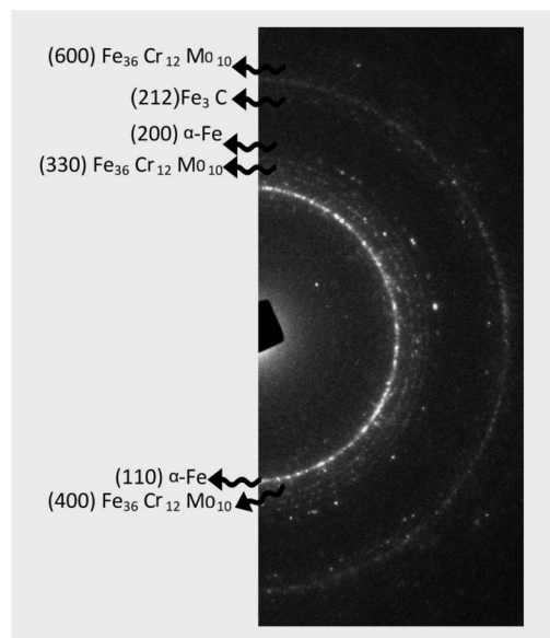
Fig. 6. Selected area diffraction pattern (SAD) for the ribbons heat treated at 850°C for 3 hours.
